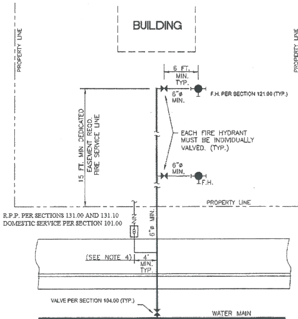
CASE II FIRE SERVICE WITH HYDRANTS ONLY
